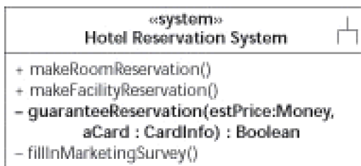
Figure 11-3: Use cases as system operations.
