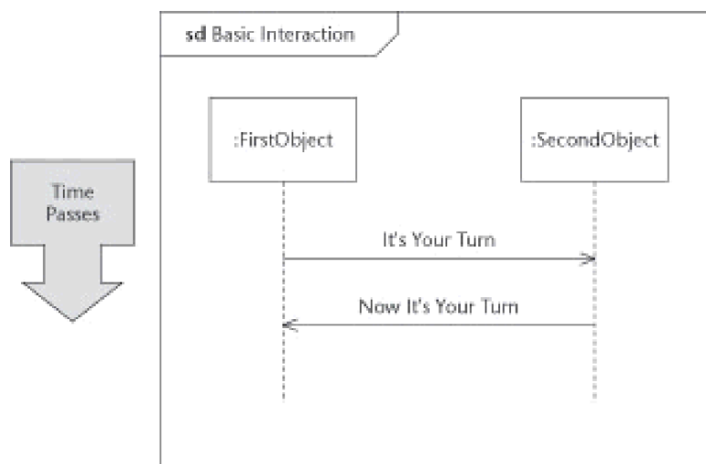
Figure 12-1: A basic sequence diagram.
