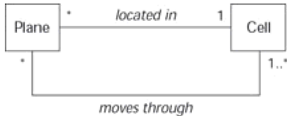
Figure 4-7: Multiplicity example with cells and planes.
