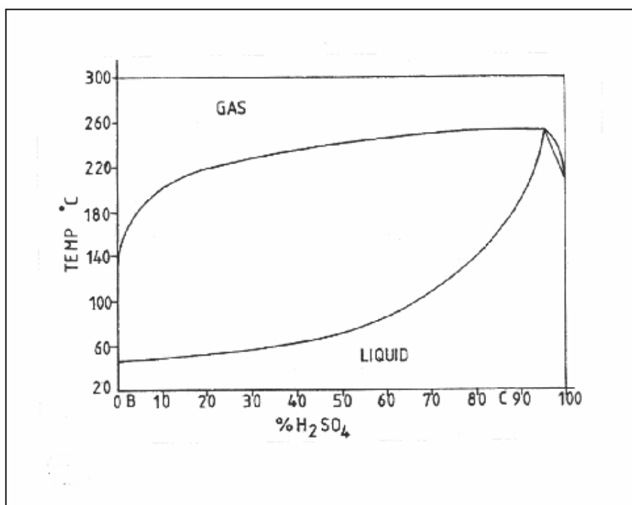
Figure 9. Phase diagram of sulphuric acid Land 3 ( P_{H_2O} + P_{H_2SO_4} = 0.1 \text{ atm} )
