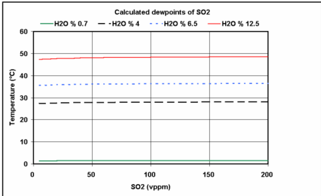
Figure 3. Dew points of \text{SO}_2 at various water contents of the gas, calculated from the formula of Kiang. The \text{SO}_2 dew points for all gasses are lower than the water dew point of the gasses.
